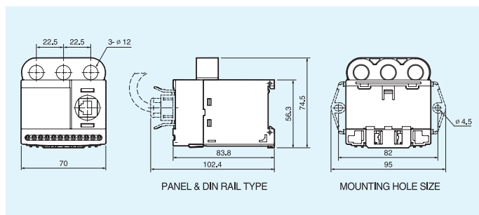
EOCR-iFDM (穿線式)
