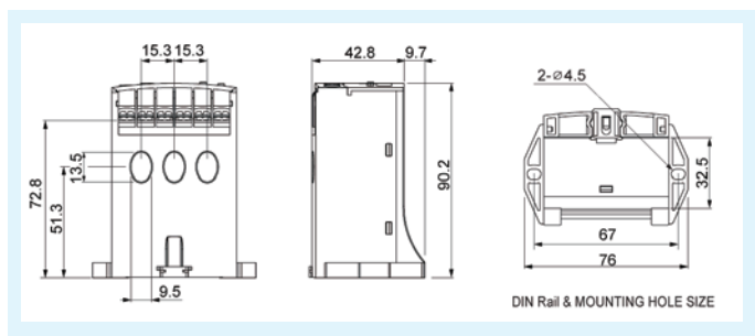
EOCR-SE2
