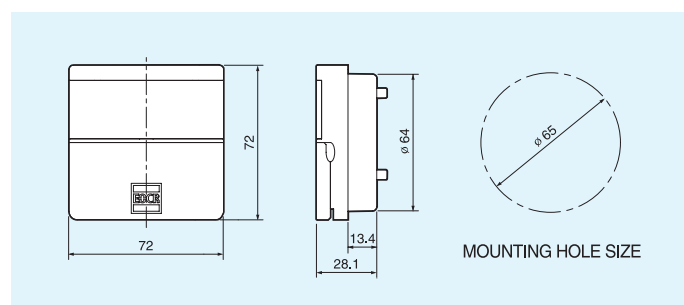
EOCR-PDM (Display)
