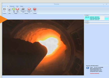
→ Flame visualization and temperature measurement
