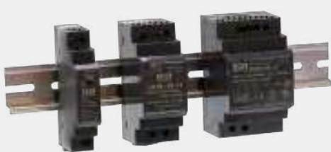
DDR-15 17.5x90x54.5 DDR-30 35x90x54.5 DDR-60 52.5x90x54.5
