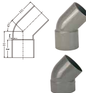
45° L 型單放口接頭 45° Elbow with Spigot End
