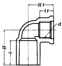
龍L接頭(塑膠牙) Faucet Fitting (Plastic Thread) — 90° Elbow
