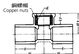
龍T入銅接頭 Faucet Fitting (Insert Bronze Nut) — Fixture Tee
