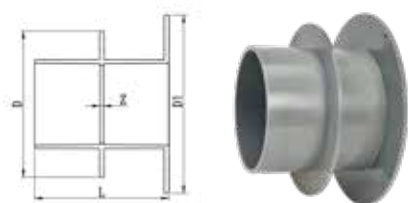
雙層止水板接頭 Coupling with Double Waterstop Board
