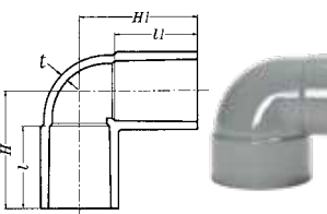
90° L 型異徑接頭 90° Reducer Elbow
