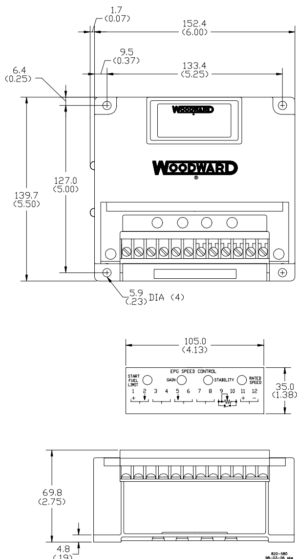
4024 Control Box Outline
