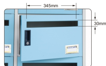
DF-MB-06L A / C W900 × D510 × H1802(mm) $24200 (118-1)
