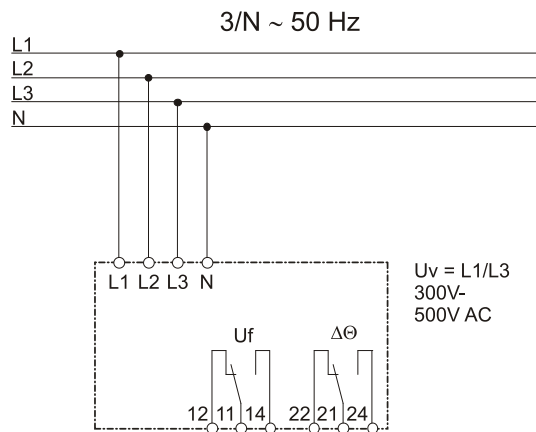
Figure 2.1: Connection four-wire system
