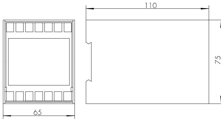
Figure 5.1: Dimensional drawings
