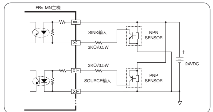
5VDC雙端輸入轉24VDC單端SINK或SOURCE輸入接線(max.200KHz)
