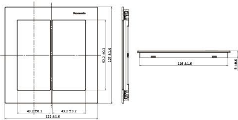
埋入式USB Power Delivery智能快速充電插座2孔
