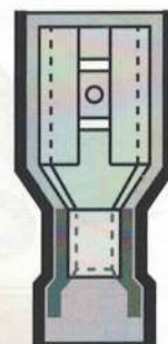
Vinyl(Nylon) Fully Insulated W/easy-Entry Copper Sleeve PVC(尼龍)全絕緣易進式銅套端子 Ex: PV(N) 1.25-7AC
