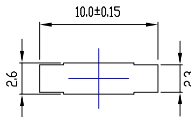
TPI NO.: SRM5001-S
